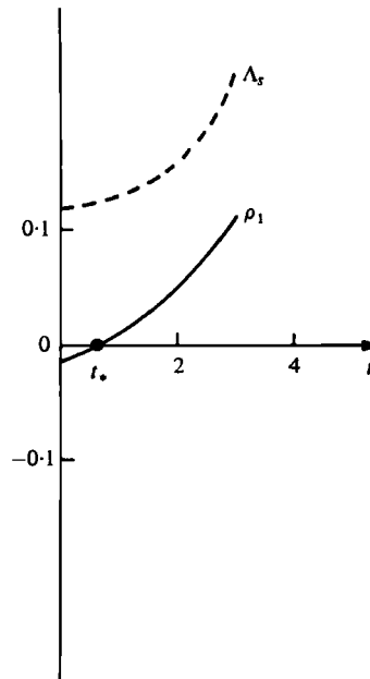
FIGURE 6. Eigenvalues \Lambda_s(t) - - - and \rho_1(t) — for La = 0.01 and Ri = 0 , calculated for N = 1 . The time t_* is designated in the text as an upper bound for the onset time for instability for this (La, Ri) pair.
